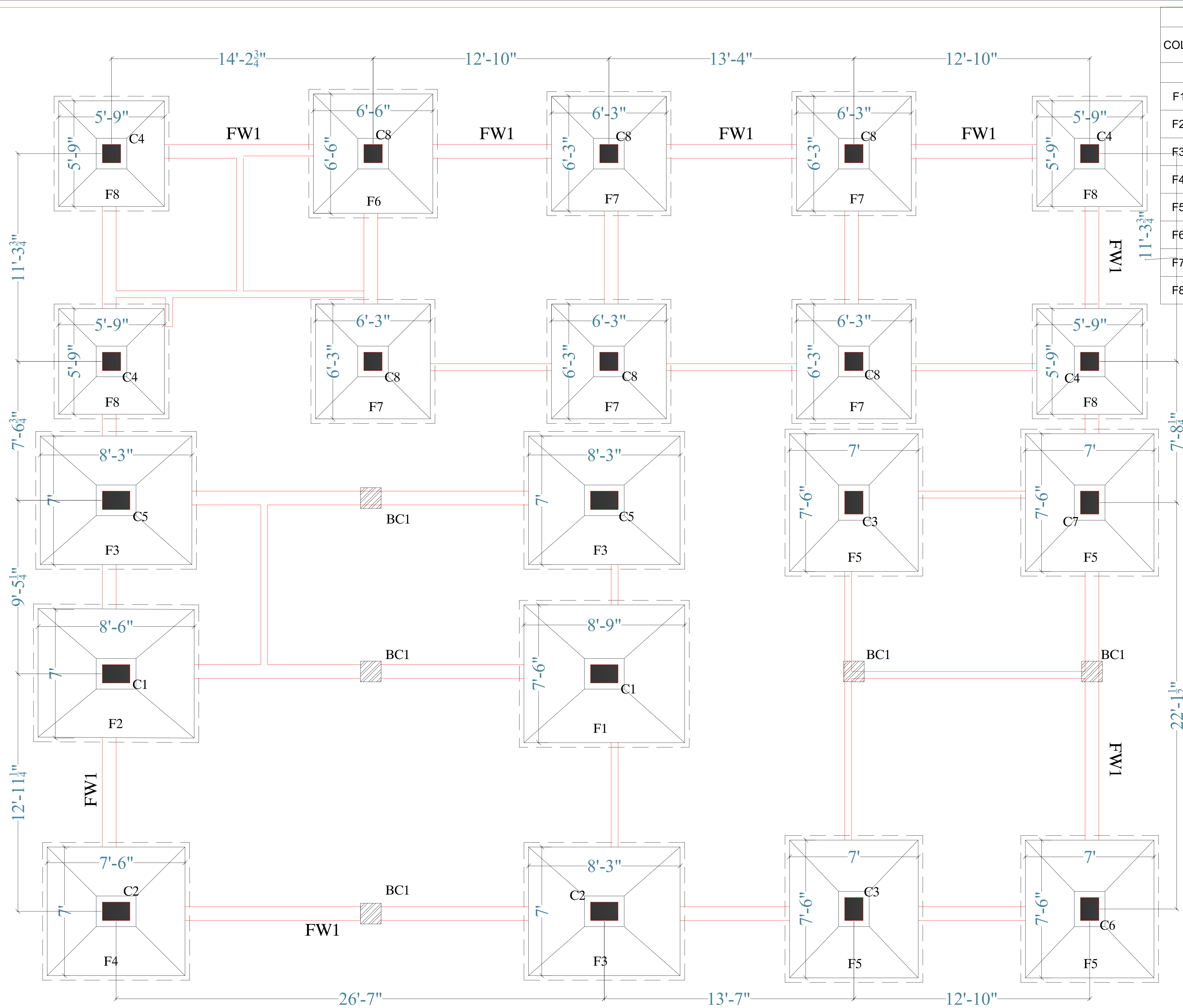
FOUNDATION LAYOUT PLAN
